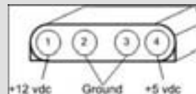
Figure 1-5: Measure the voltages on the power connector.
