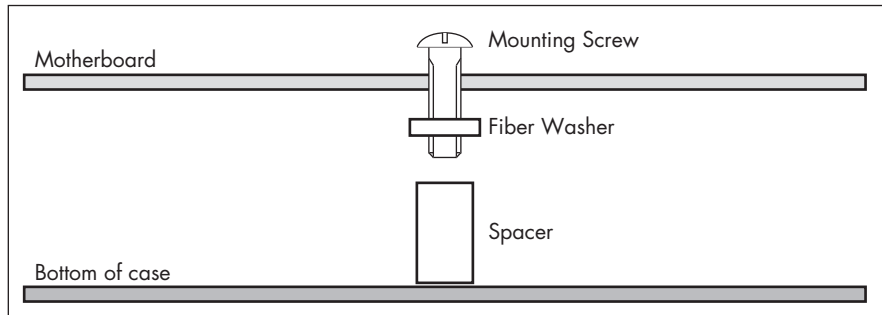
Figure 17-2: Use fiber washers to insulate the motherboard from the bottom of the computer's case.
